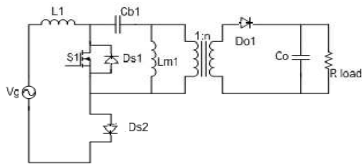
Figure 3. The proposed operated at positive
