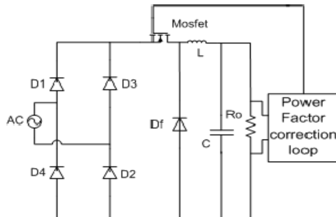
Figure 1. Two Stage AC-DC PFC
