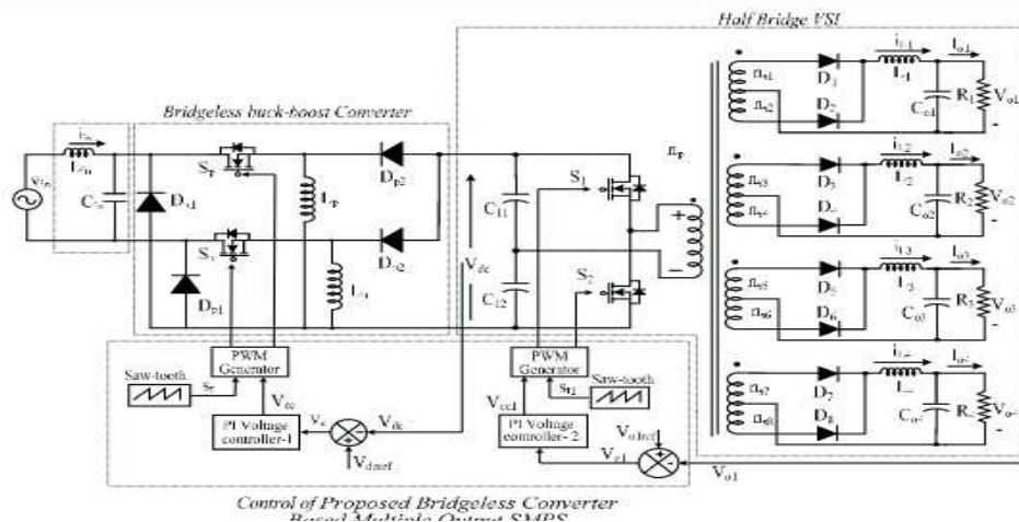
Figure 4-Bridgeless converter based multiple output SMPS
