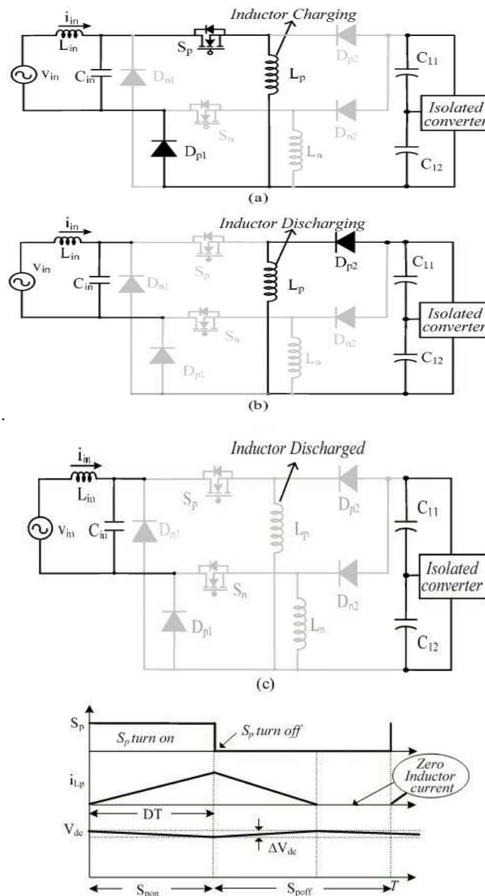
Figure 5. Operating modes for under (a) upper switch S_p is on, (b) upper switch S_p is off, (c) both switch and diode are off, (d) wave forms in one switching cycle
