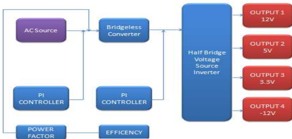
Figure 6. Block diagram implementing PI Controller
