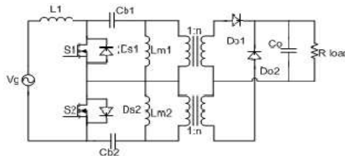
Figure 2. The Proposed Converter
